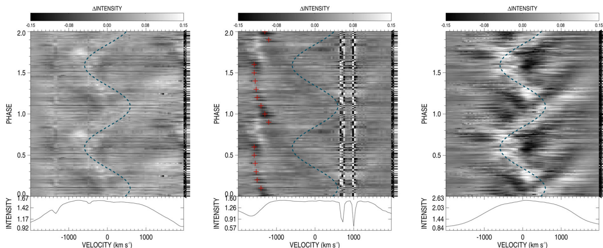
Figure 11. The phased difference grey-scale images of the C IV \lambda\lambda 5802,5812 doublet, with a mean wavelength of \lambda 5806 adopted (left), the He I \lambda 5876 (centre) and He II \lambda 5411 (right) emission lines during the second 40-d period of the campaign. The DAC-like feature is outlined (red crosses) at negative velocities in the He I \lambda 5876 line. The dashed blue line represents the kinematics model calculated in Section 4.2.
