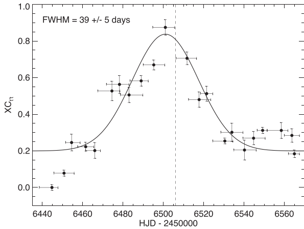
Figure 8. The cross-correlation analysis for the centre reference image (dashed vertical line). The x-axis error bars show the time covered by each image, while the y-axis error bars display the XC_{t,t} errors. The solid line is the Gaussian function that was fitted for the analysis. The remaining two cross-correlation images are located in Appendix A, Figs A23–A25 (online only).
